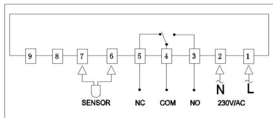
Water Heating System
