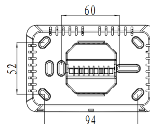
Mounting Hole (unit:mm)
